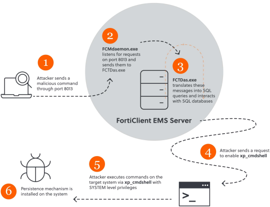
Figure 3. Supply chain Ransomware Attack - Fortigate Medusa attack
